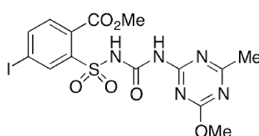
Iodosulfuron-methyl
