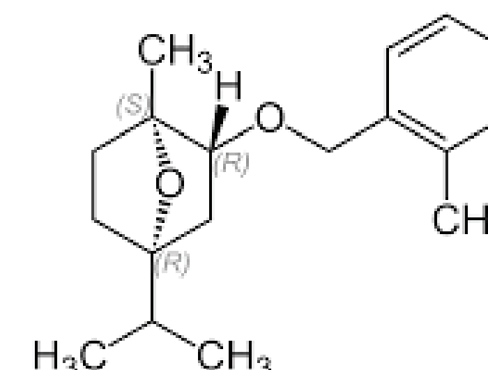
Cinmethylin
