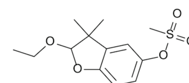
Ethofumesate
