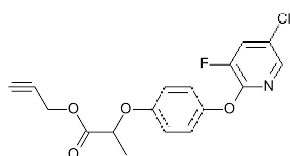
Clodinafop-propargyl
