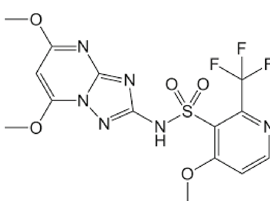
Thienencarbazone-methyl
