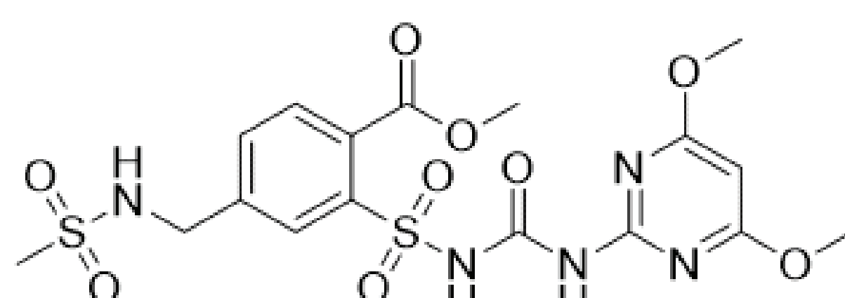
Mesosulfuron-methyl
