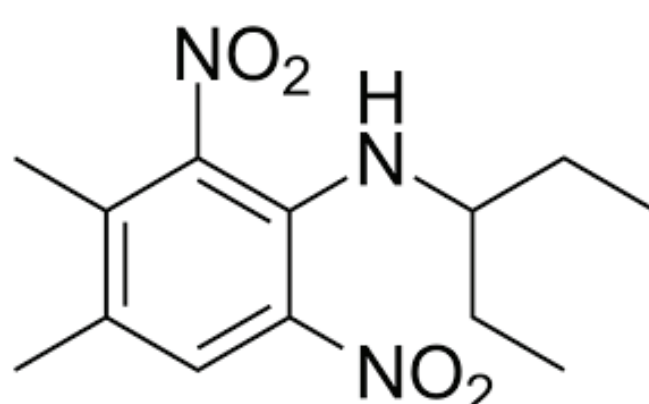
Pendimethalin
