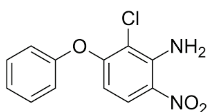
Aclonifen
