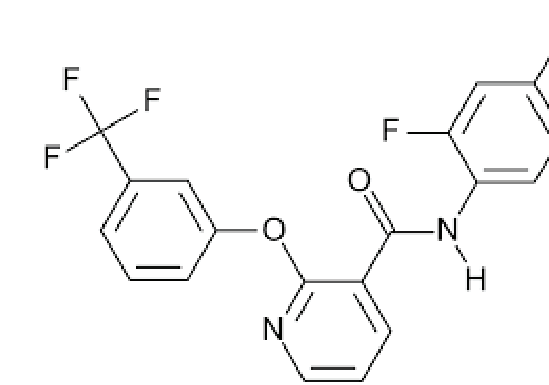
Diflufenican
